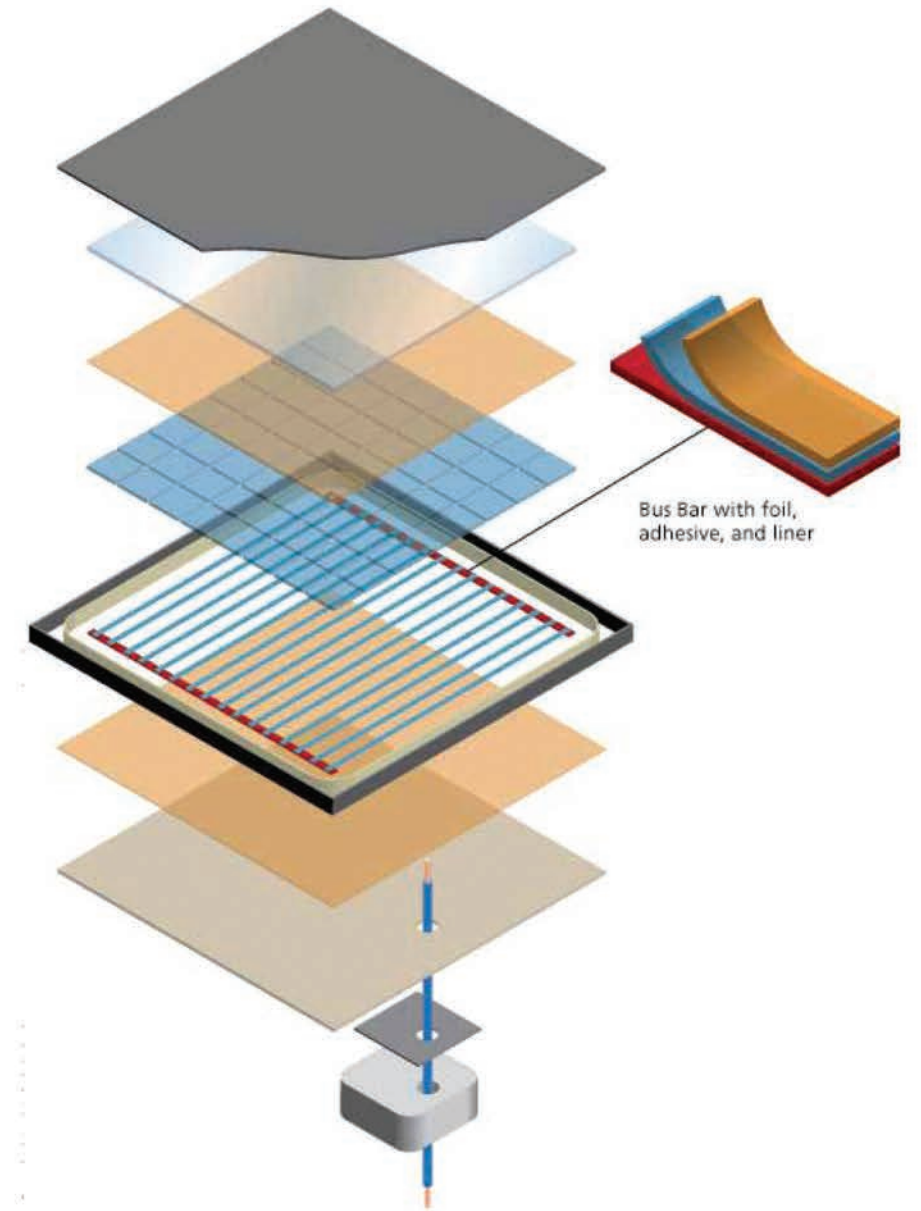
Bus bar illustration.
